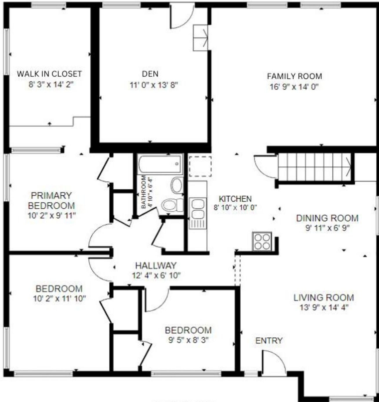
MAIN FLOOR
